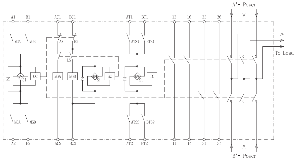
Circuit Diagram (회로도) 800A~1600A
