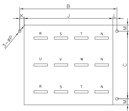
PANEL CUTTING
