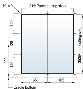
&lt;Mounting hole&gt;
