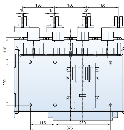
4P
