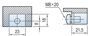
Terminal section
