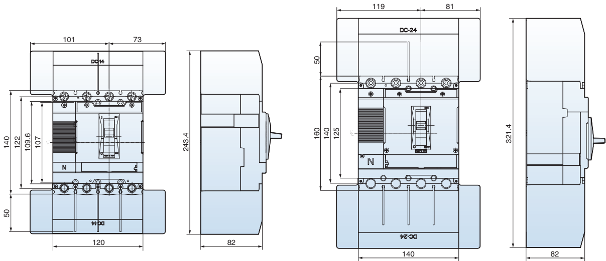
4P (L-type)
