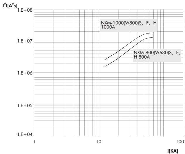
800 (W630)/1000 (W800) frame let-through current curve
