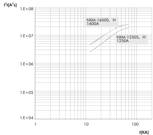
1250/1600 frame let-through current curve
