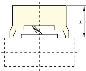
Installation sketch of electric operational mechanism
