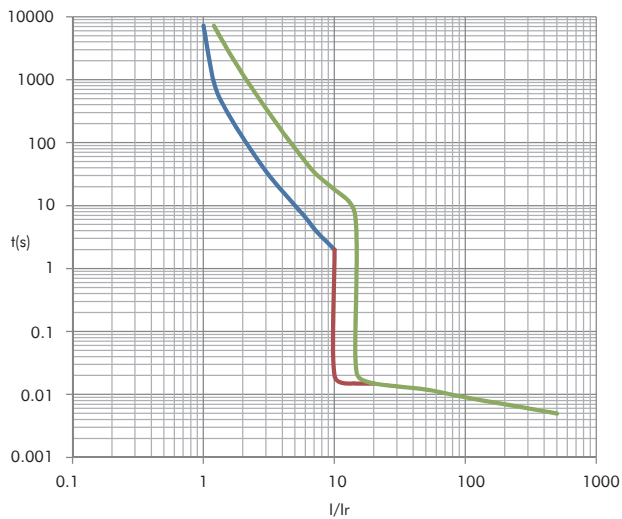
Tripping curve of motor protection
