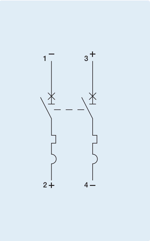
Two pole series connection diagram
