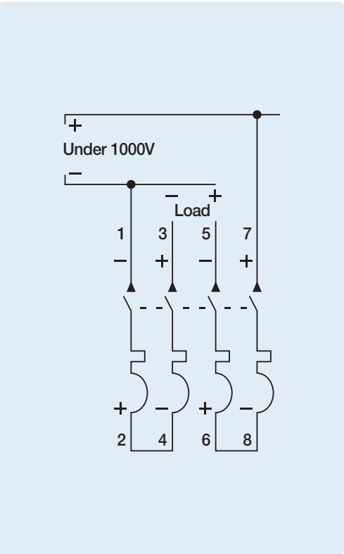
Four pole series connection diagram
