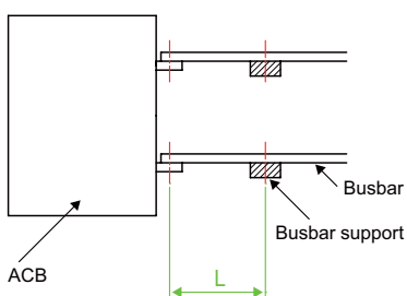
Horizontal terminals
